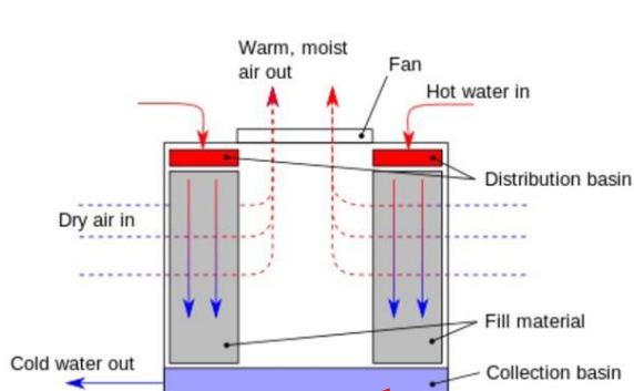
Cross-Flow Cooling Tower
