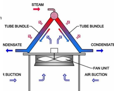
Dry Cooling Tower
