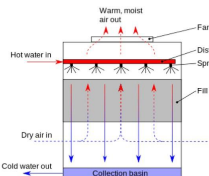
Counterflow Cooling Tower
